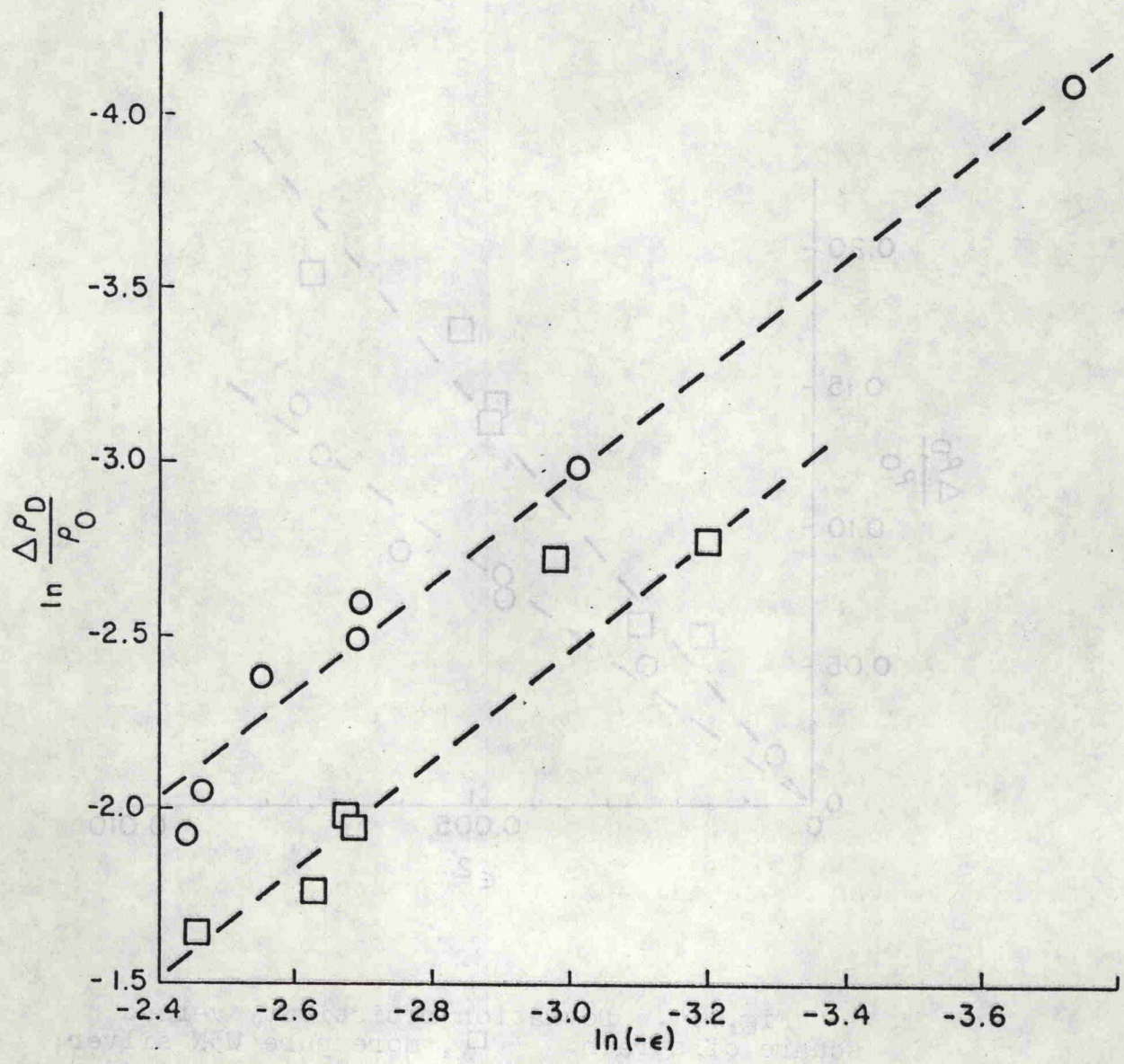
Fig. 15. Logarithmic plot of deviation resistivity versus strain. □, more pure W3N silver; ○, MRC silver.
